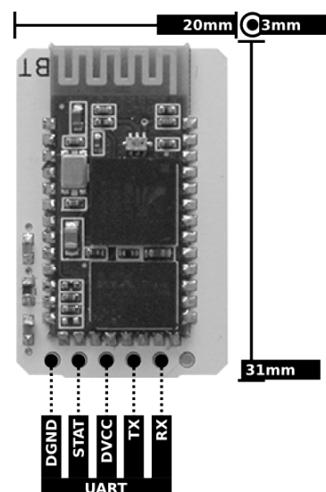
Fig. 1. Pin-out and physical dimensions.
