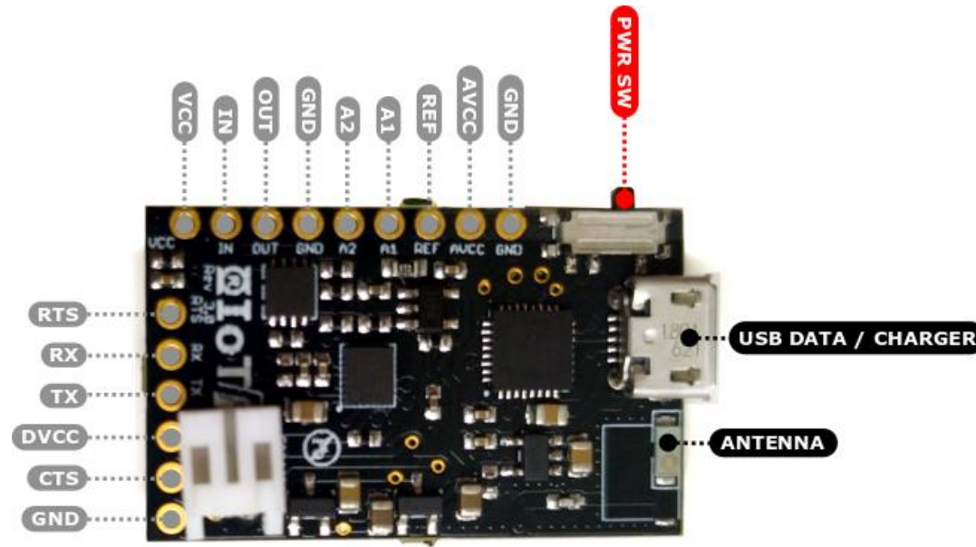
Fig. 4. Pinout and other main components.
