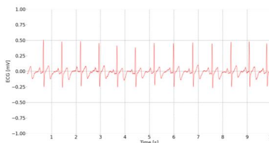
Fig. 3. Typical raw ECG data (acquired with BITalino (r)evolution) using an Einthoven triangle configuration.
